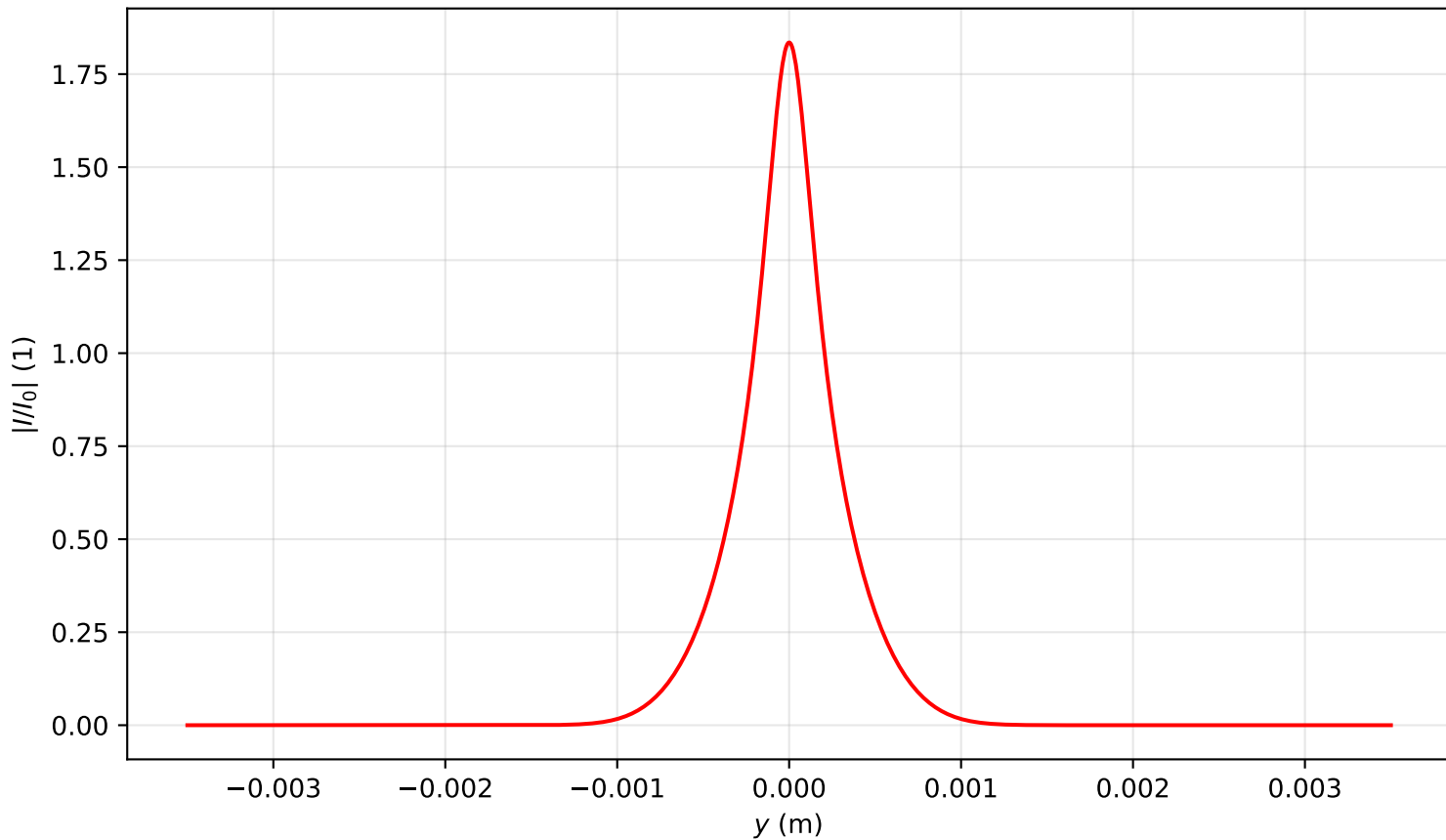
Intensity profile I(x=0, y, z=0.239)/I_0 , P_{in}=7.5P_{cr} , artificial time
